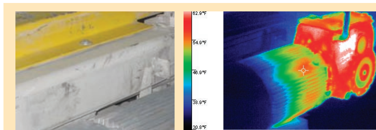
Figure 6. This thermal image shows a cool motor on the left and a hot gearbox on the right, with an especially white-hot anomaly.
