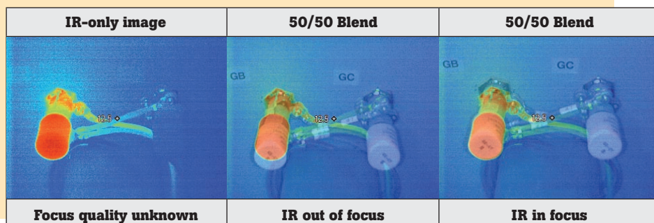
Figure 8. Fusion can help in focusing an infrared image by adjusting the focus until the IR and visible images match
