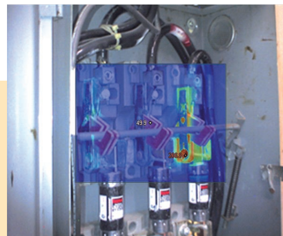
Figure 5. Putting camera image into the picture-in-picture mode helps further identify problem location
